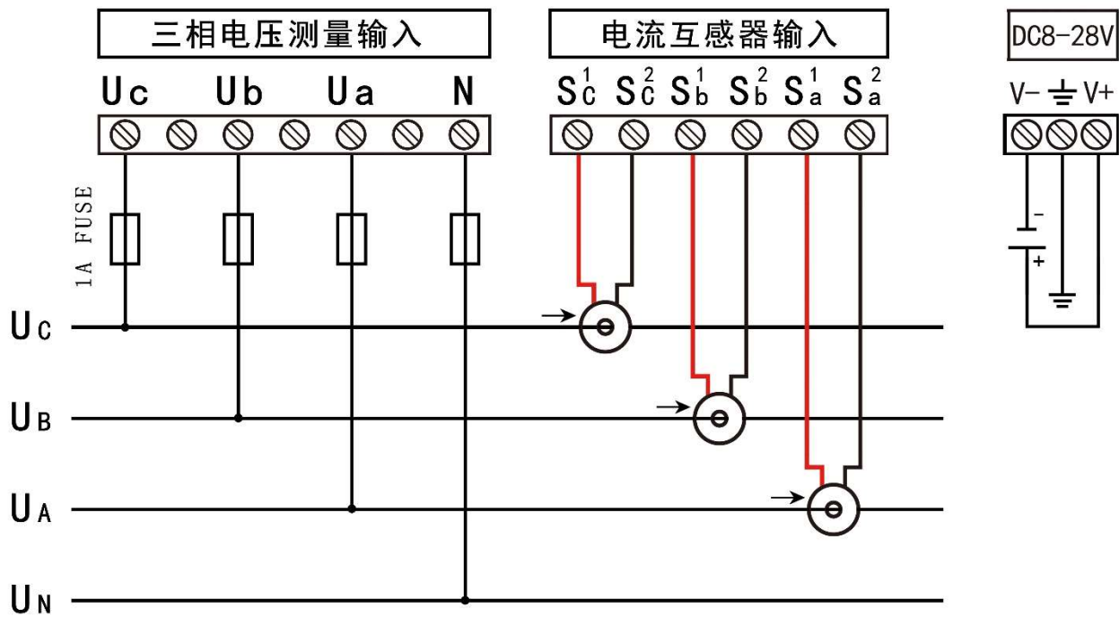
HD250VXXA3GK-D接线图
